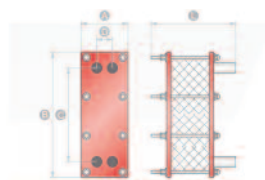
Dimensiones G-12 N (mm) A [180] B [480] C [357] D [60] L [de 6 a 30 placas] [240] L [de 32 a 50 placas] [320]
