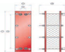
Dimensiones GC-8 (mm) A [180] B [762] C [640] D [60] L [de 6 a 50 placas] [225]
