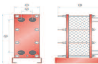
Dimensiones G-30 P (mm) A [270] B [760] C [555] D [100] L [de 6 a 48 placas] [360]
